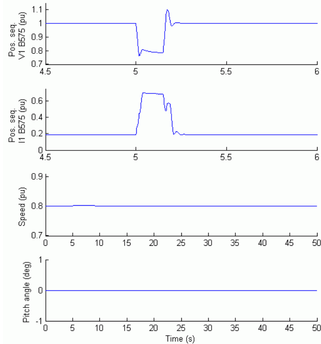
Wind Farm Waveforms During Fault at Bus B25 (Wind Farm in Voltage Regulation Mode)
