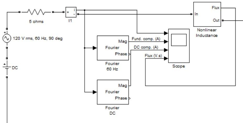
Implementation of a Nonlinear Inductance
