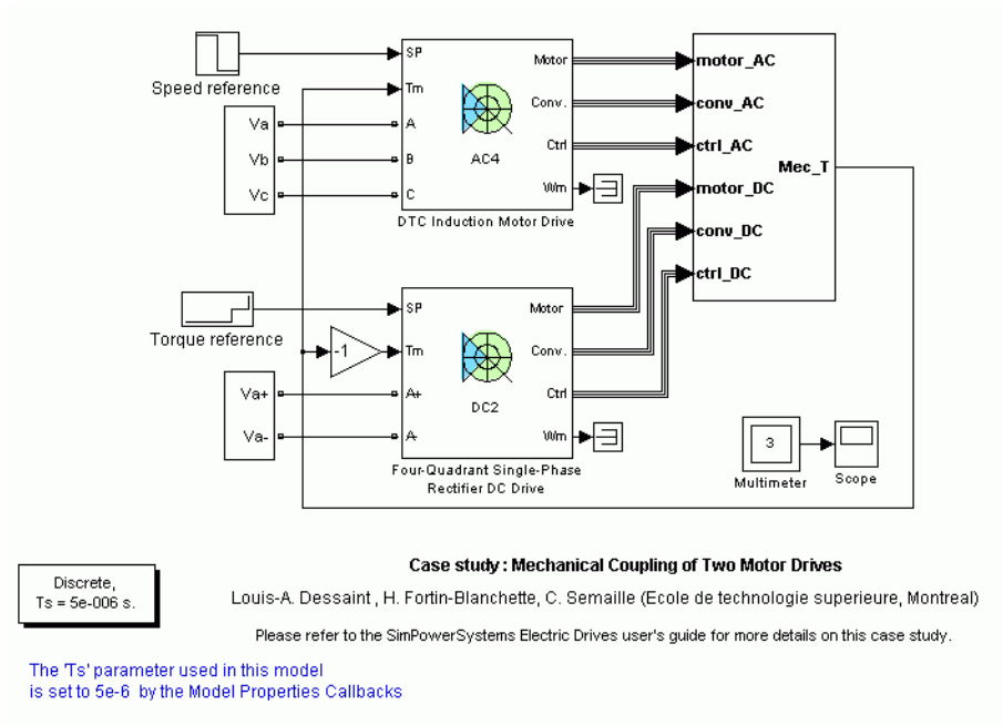
SPS Diagram of the Two Interconnected Drives
