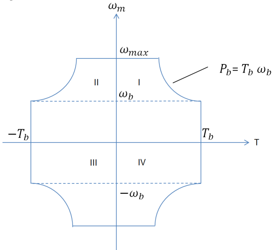
Four-Quadrant Operation of an Electric Drive
