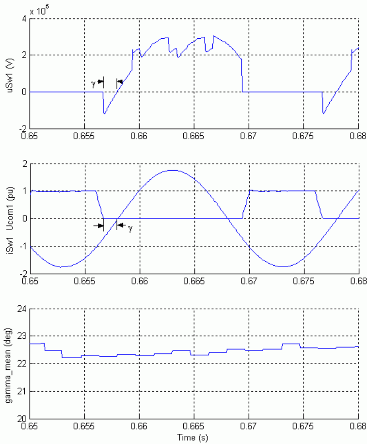
Current and Commutation Voltage of Valve 1 Showing \gamma
